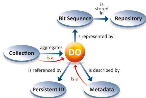
Figure 2 This figure indicates the core data model as it was worked out within the RDA group Data Foundation and Terminology (DFT).
