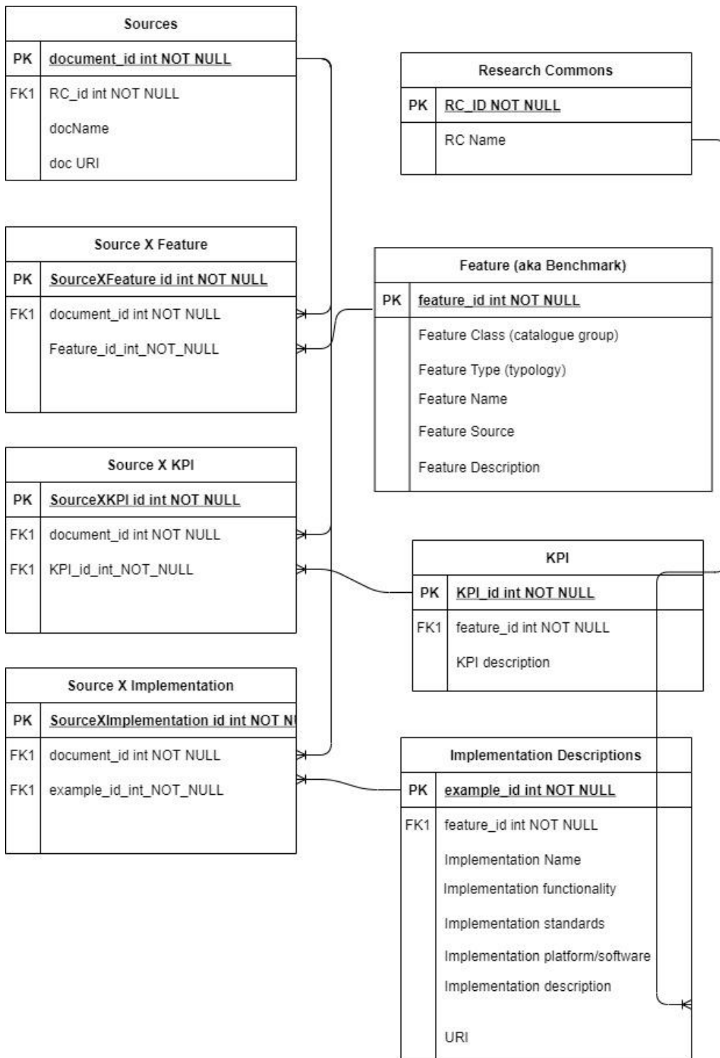
Figure 2. Draft UML for a database used to capture attributes.
