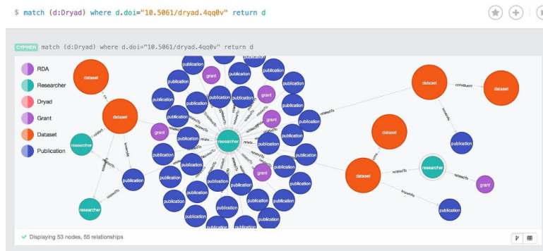
Figure 1: RD-Switchboard interface to the graph database using Neo4j
